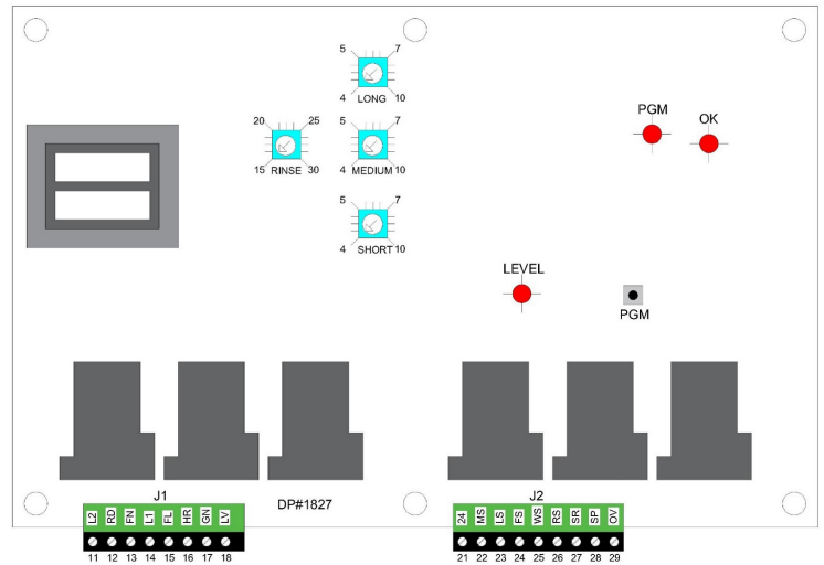
Douglas Control Board, Part # 1827
