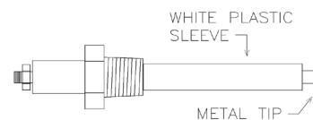
Water Probe (Low Water Protection)
